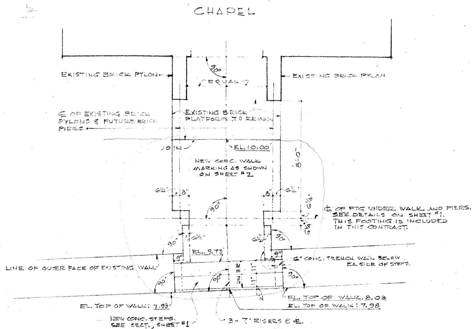
PLAN OF WORK IN THIS CONTRACT SCALE: 1/4" = 1'-0"
